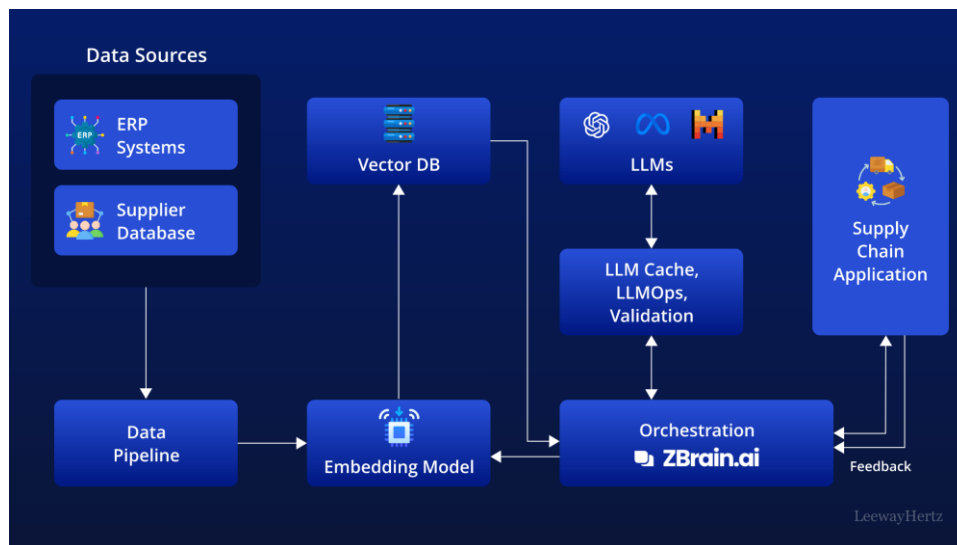
Fig. 1: AI Driven Semantic Analytics and Cloud Orchestration
