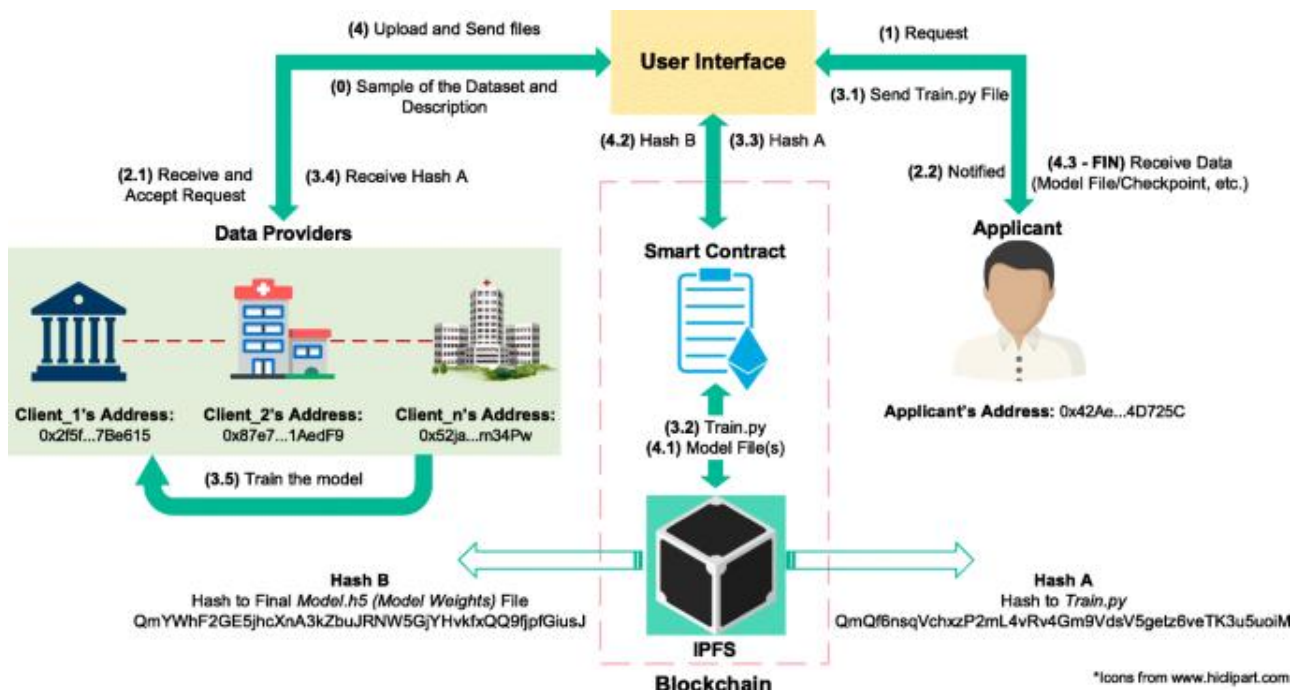
Fig.1. Privacy-preserving federated learning for scalable and high data quality computational-intelligence
